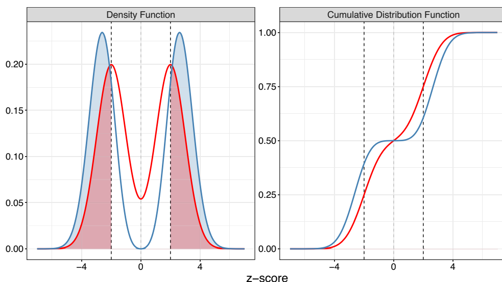
FIGURE 1 Comparison between local (red) and non-local (blue) distributions. The acceptance region \mathcal{A} = [-2, 2] is highlighted by vertical dashed lines. The left panel compares the density functions, the right one the c.d.f.'s. The colored areas in the left panel represent the power \mathbb{P}[Z \notin \mathcal{A}|H_1]
