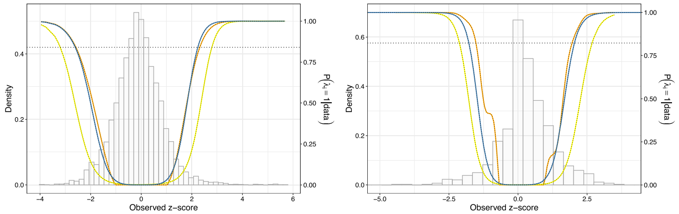
FIGURE 4 HIV (left) and Torondel (right) datasets. Histograms of the data with function P_1(z) superimposed computed via the \text{LocFDR} (orange), the \text{MixFDR} (yellow) and Nollik (blue). The horizontal dotted lines represent the estimated threshold controlling for a BFDR of 5%
