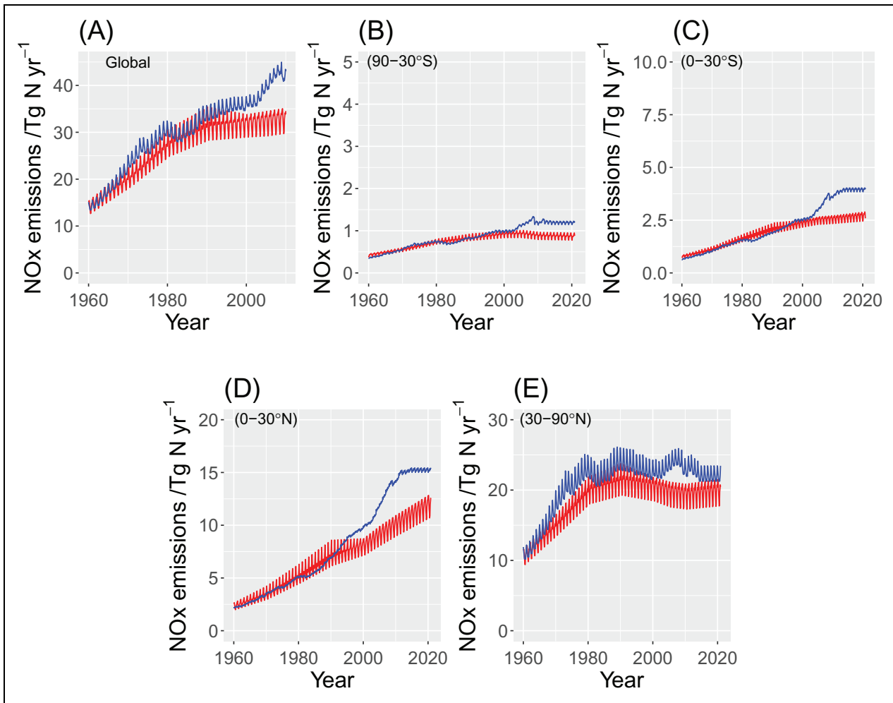
Figure 8. Anthropogenic (land based) NO x emissions (blue) from the bottom-up Community Emissions Database System inventory (Hoesly et al., 2018) for the period 1960–2010 and (red) from the MACCity implementation of the CMIP5 emissions inventory of Lamarque et al. (2010) through 2000 and the RCP8.5 scenario thereafter (as used in the Chemistry Climate Model Initiative simulations; Granier et al., 2011). Panels B–D show the same latitude regions as analyzed in Figure 9 . DOI: https://doi.org/10.1525/elementa.2020.034.f8
