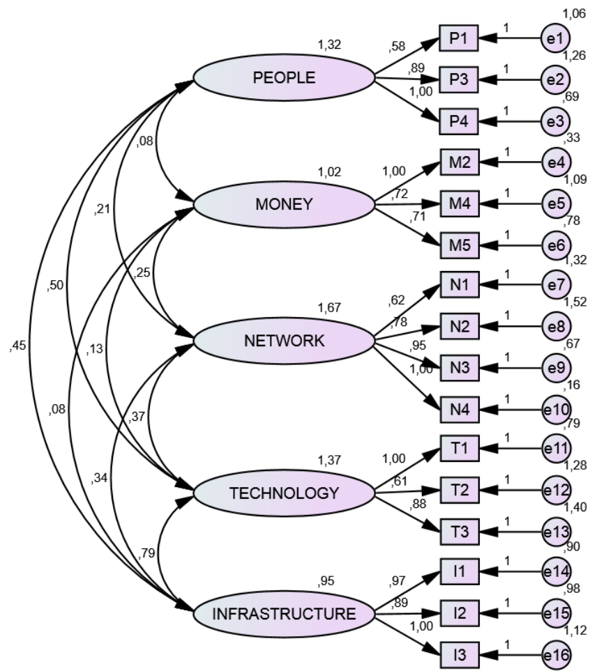
Figure 3. Factor model, with factor loadings, variances and covariances.
