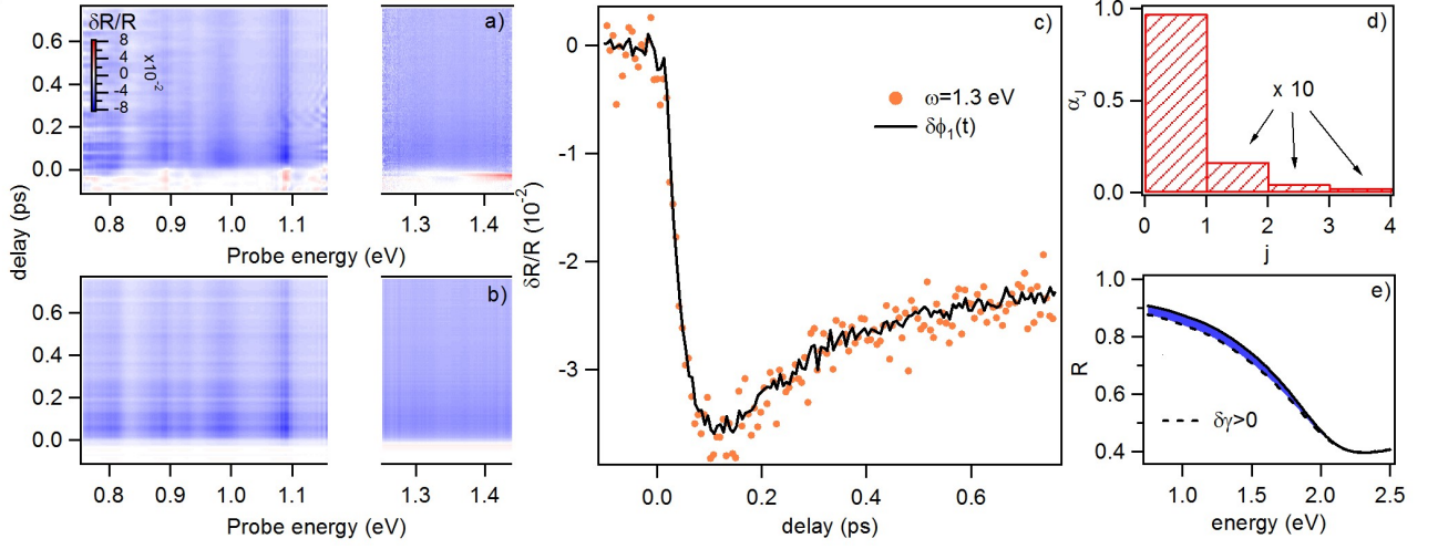
FIG. S5: a,b) \text{MgB}_2 transient reflectivity variation compared with the matrix calculated as the outer product between \Psi_1(\omega) and \delta\phi_1(t) multiplied by the first singular value k_1 c) Time trace at \hbar\omega=1.3 eV displayed with the first temporal eigenvector \delta\phi_1(t) weighted by \Psi_1(\omega=1.3 eV) and k_1 d) Weights \alpha_j of the singular values normalized to one ( \alpha_j = \frac{k_j^2}{\sum_j k_j^2} ) and sorted in decreasing order e) \text{MgB}_2 in plane static reflectivity measured at T=300 K (black line) and the static reflectivity calculated within the framework of the EDM by simulating an increase of the scattering rate (dashed line).
