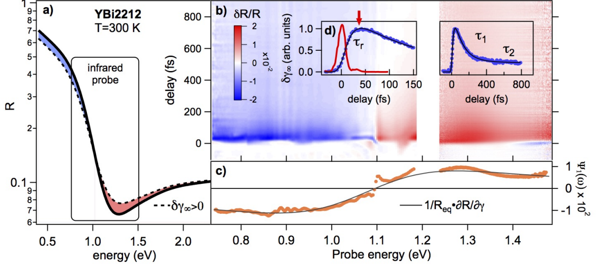
FIG. 1: Equilibrium and non-equilibrium optical properties of YBi2212. a) The normal state reflectivity (black line) of the YBi2212 crystal is reported. The dashed line represents the reflectivity calculated by increasing the electron-boson scattering rate, \gamma_\infty , in the extended Drude model. b) The ultrafast dynamics of \delta R/R(\omega, t) , measured across the isosbestic point \tilde{\omega} , is reported. The measurements have been performed with an incident pump fluence of 0.7 \text{ mJ/cm}^2 . The linearity of the optical response has been checked in the 0.2\text{-}2 \text{ mJ/cm}^2 fluence range. c) The first eigenfunction, \Psi_1(\omega) , obtained through the SVD (see Supplementary Information) is displayed (yellow dots). SVD consists of decomposing \delta R(\omega, t)/R_{eq}(\omega) \simeq \sum_k \Psi_k(\omega) \delta \phi_k(t) . The fit obtained by increasing the total scattering rate, i.e., \Psi_1(\omega) = 1/R_{eq}(\omega) \cdot \partial R / \partial \gamma(\omega) , is reported as a black line. d) The time-dependent scattering rate variation, \delta \gamma_\infty(t) = \delta \phi_1(t) , is reported (blue dots). The black line is the fit to the data of the function (1 - \exp(-t/\tau_r)) \cdot (I_1 \exp(-t/\tau_1) + I_2 \exp(-t/\tau_2)) convoluted with a gaussian pulse accounting for the experimental time-resolution. The red line is the measured cross-correlation trace between the pump and probe pulses, that sets the time-resolution to 19 \pm 2 fs. The red arrow highlights the time delay ( \sim 40 fs) at which the maximal \delta \gamma_\infty variation is measured.
