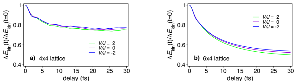
FIG. S8: Kinetic energy \Delta E_{\text{kin}}(t)/\Delta E_{\text{kin}}(t=0) in the system of two carriers, for different values of the direct carrier-carrier interaction V , see Eq. (S9). The other parameters are the same as in Fig. 2 of the main text, i.e., J/t_h = 0.3 , t_h = 360 meV and \Delta E_{\text{kin}}(t=0) = 2 eV. Results have been obtained by exact diagonalization on a) 4 \times 4 and b) 6 \times 4 square lattice using periodic boundary conditions.
