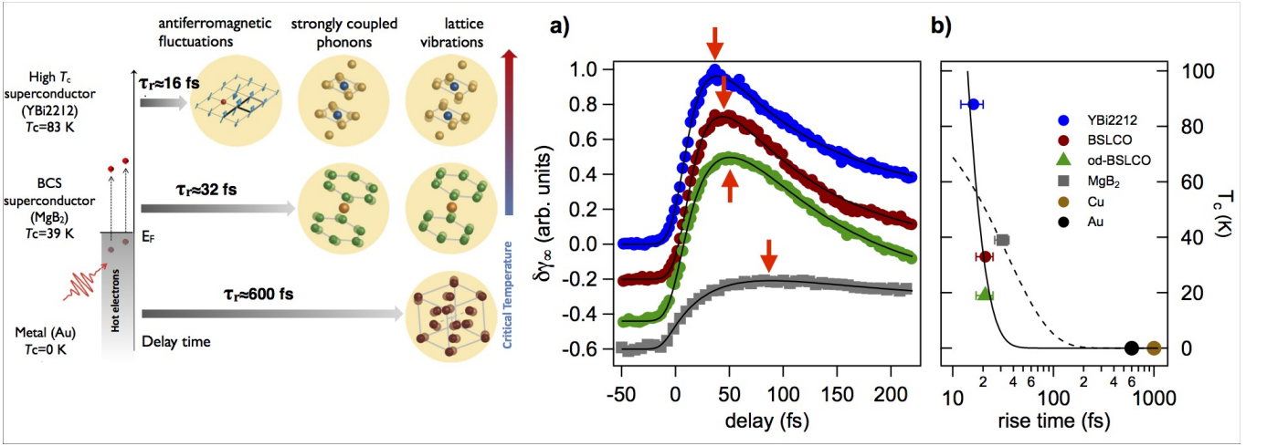
FIG. 3: Ultrafast dynamics of the electron-boson interaction. The different relaxation dynamics in high- T_c superconductor and in conventional superconductors are sketched in the left panel. a) The dynamics of \delta\gamma_\infty(t) is shown for different superconducting systems (YBi2212, blue circles; BSLCO, red circles; od-BSLCO, green circles; \text{MgB}_2 , grey squares). The red arrows highlight the time delay corresponding to the maximal value of \delta\gamma_\infty(t) after the excitation. b) The critical temperatures of the systems considered is reported as a function of the build-up time ( \tau_r ) of \delta\gamma_\infty(t) , measured through the time-resolved optical spectroscopy. The black lines are the critical temperatures calculated by the Eliashberg-like expression T_c=0.83\tilde{\Omega}\exp[-1.04(1+\lambda_b)]/[\lambda_b-\mu^*(1+0.62\lambda_b)] [26], fixing \mu^*=0 and assuming a generic relation between the electron-boson energy exchange rate, 1/\tau_r , in cuprates and the total coupling constant \lambda_b and \tilde{\Omega}=200 meV (solid line). The dashed line represents the critical temperatures calculated for \tilde{\Omega}=70 meV and \lambda_b=1.1 compatible with the phonon-mediated pairing in \text{MgB}_2 [11].
