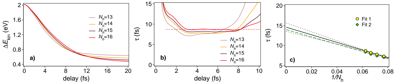
FIG. S7: a) Kinetic energy of a photo-excited hole, \Delta E_{\text{kin}}(t) , for different sizes of the functional space, given by the parameter N_h . b) The function \tau(t) = -\Delta E_{\text{kin}}(t)/\Delta \dot{E}_{\text{kin}}(t) , where \Delta \dot{E}_{\text{kin}}(t) denotes time-derivative, for the same system sizes. Horizontal dashed line indicates the plateau for N_h = 16 where \tau(t) becomes time-independent. c) \tau vs 1/N_h for two different fitting procedures. In Fit 1, we extract \tau^{(1)}(N_h) from a time-independent plateau of \tau(t) , as indicated in panel b). In Fit 2, we extract \tau^{(2)}(N_h) from a fitting function f_2(t) = A_0 \exp(-\sqrt{at^2 + b^2} + b) . Details are described in the main text. Both fitting procedures yield a very similar relaxation time, \tau_{t,J} \approx 15 fs. Dotted lines represent extrapolation for Fit 1, with fitting parameters shifted by 3 standard deviations relative to the mean values.
