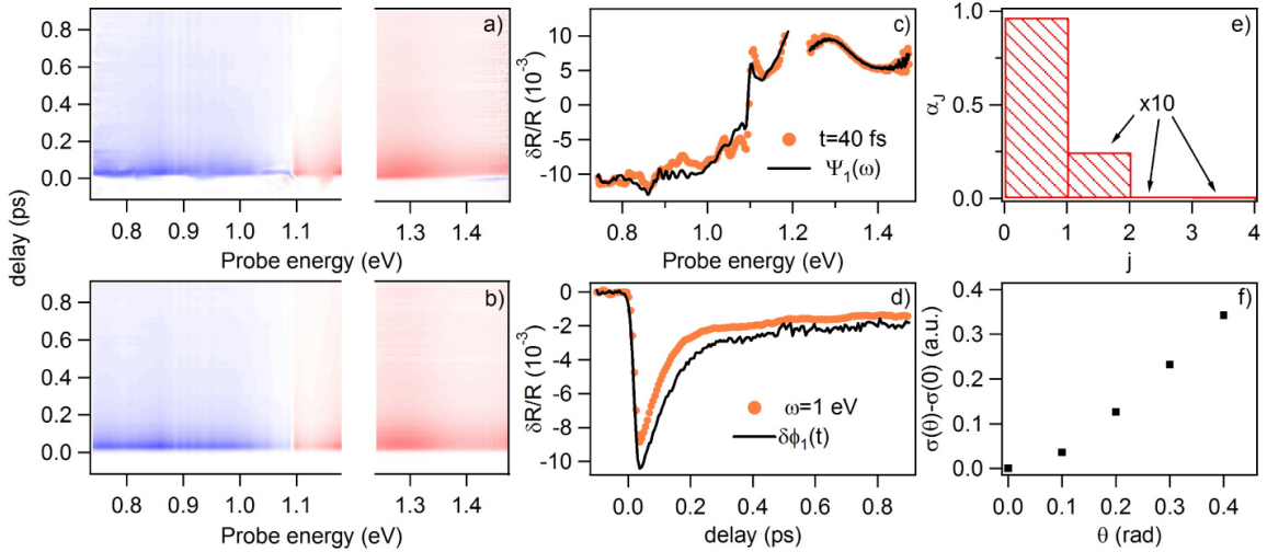
FIG. S1: a) Transient reflectivity variation of Y-Bi2212 UD . b) Time-frequency matrix calculated as the outer product between \Psi_1(\omega) and \delta\phi_1(t) multiplied by the first singular value k_1 c) Energy trace at t=40 fs, corresponding to the maximum variation of the transient signal, (orange dots) and the first spectral eigenvector (black line) \Psi_1(\omega) multiplied by \delta\phi_1(t=40 fs) and k_1 d) Time trace at \hbar\omega=1 eV displayed with the first temporal eigenvector \delta\phi_1(t) weighted by \Psi_1(\omega=1 eV) and k_1 . For graphical reasons, \delta\phi_1(t) has been offset. e) Weights \alpha_j of the singular values normalized to one ( \alpha_j = \frac{k_j^2}{\sum_j k_j^2} ) and sorted in decreasing order f) \sigma(\theta) , defined in Eq. S2, computed for different value of the rotation angle \theta .
