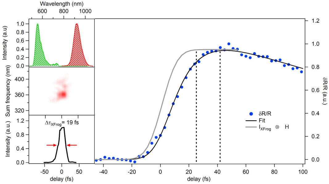
FIG. S6: a) Spectrum of the pump (OPA3) and the probe (OPA2) pulses; b) Measured XFROG trace; c) Cutoff of the XFROG trace taken at the maximum of the signal (360 nm); d) Transient reflectivity at \lambda_{\text{probe}}=930 nm (blue dots), fit of the data (black line), convolution between Heaviside function H and the XFROG trace at I_{\text{XFROG}} (grey line).
