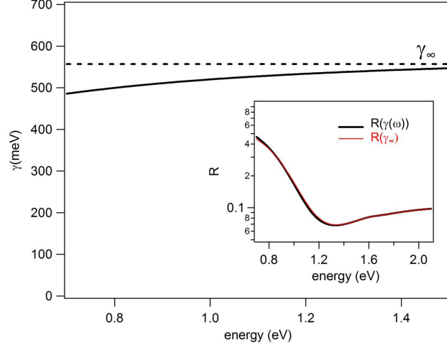
FIG. S3: Energy dependence of the scattering rate at T=300 K in the probe spectral range. \gamma_\infty is the asymptotic value of the scattering rate. In the inset the EDM fit to static reflectivity (black line) is compared with the calculated reflectivity (red line) under the frequency independent approximation of the damping term: \gamma(\omega) = \gamma_\infty .
