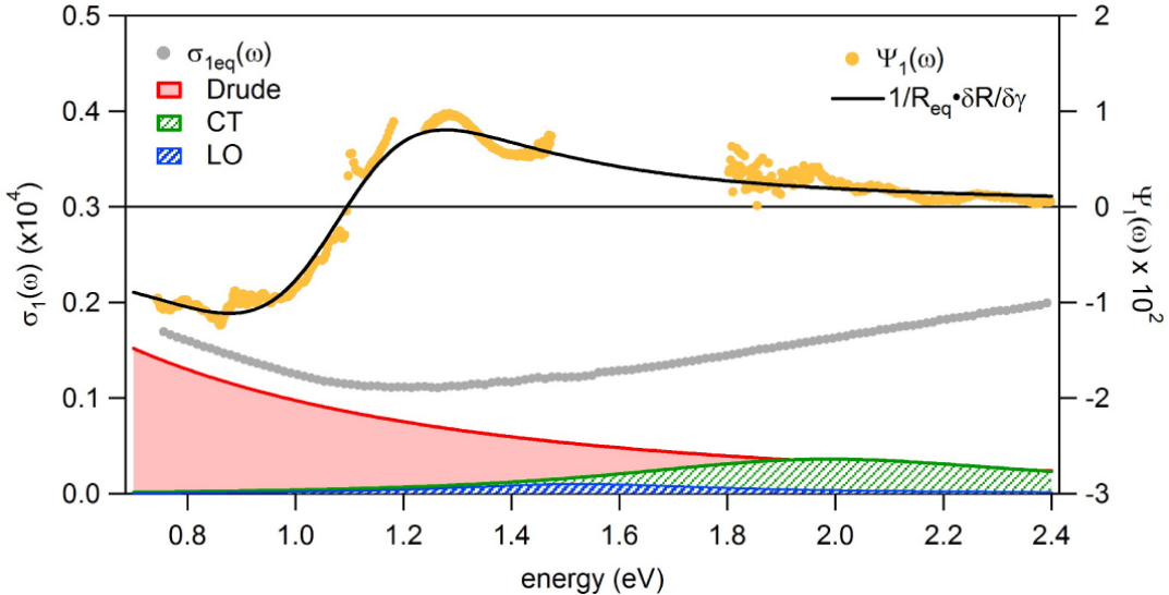
FIG. S4: The experimental equilibrium optical conductivity (grey dots) together with the Drude and charge transfer peak resulting from the fit of the equilibrium optical conductivity (red and the green lines). The first eigenvalue obtained from the SVD analysis is reported (yellow dots). The trace extending between 0.7 and 1.5 eV is the one previously reported in Fig. 1 of the main text. The trace extending between 1.8 eV and 2.4 eV results from the SVD analysis of the Y-Bi2212 UD transient response probed by NOPA 3. The black line is the best fit obtained by increasing the total scattering rate.
