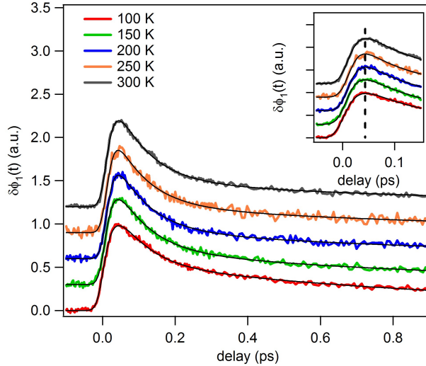
FIG. S2: Temporal dynamics of \delta\phi_1(t) eigenvectors at different temperatures. The black lines are the fit to the data. The fitting function takes into account the experimental resolution, as described more extensively in the main text. In the inset, the dynamics at short delay times clearly show that the rise time of the temporal traces does not depend on the temperature.
