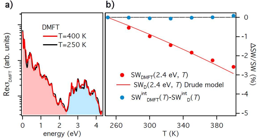
FIG. S9: a) The optical conductivity of the single band Hubbard Model calculated by DMFT is reported for T=250 and 400 K and U=3 eV. A broad Drude peak extends up to 2.4 eV, whereas the optical properties are dominated by interband transitions at the U energy scale. b) The relative variation of the optical spectral weight, i.e., \Delta\text{SW}/\text{SW} = \text{SW}_i(\Omega_c, T) - \text{SW}_i(\Omega_c, 250\text{K}) / \text{SW}(\Omega_c, 250\text{K}) , as a function of the temperature T . The temperature-dependent intraband spectral weight \text{SW}_i(2.4 \text{ eV}, T) = \int_0^{2.4\text{eV}} \text{Re}\sigma_i(\omega, T) d\omega is calculated for the DMFT optical conductivity ( i=\text{DMFT} , red dots) and for an extended Drude model ( i=D ). The interband spectral weight is calculated as the difference between \text{SW}_{\text{DMFT}}^{\text{int}}(T) = \int_{2.4\text{eV}}^{4.2\text{eV}} \text{Re}\sigma_{\text{DMFT}}(\omega, T) d\omega and the intrinsic spectral weight of the underlying Drude tail, i.e., \text{SW}_D^{\text{int}}(T) = \int_{2.4\text{eV}}^{4.2\text{eV}} \text{Re}\sigma_D(\omega, T) d\omega .
