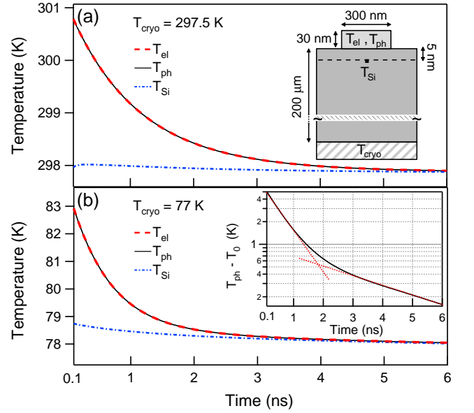
FIG. 2: (Color online) Simulations results for T_{cryo} = 297.5 and 77 K. Insets. Panel (a): locations within the sample where the temperatures are calculated. Panel (b): the difference between T_{ph} and its asymptotic value T_0 , in semi-log scale; dashed red lines are a guide to the eye, showing double exponential behavior.
