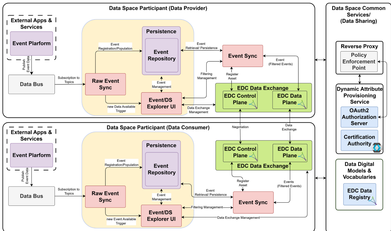
Figure 2. NSCA Data space architecture.
