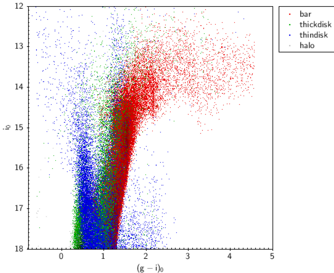
Figure 7. A model CMD of the population towards Baade’s Window ( l, b = (-0.2^\circ, +3.9^\circ) covering 0.1 \text{ deg}^2 (see text and the Besancon Galaxy Model; Lagarde et al. 2017)). This model breaks down the the CMD by stellar populations as indicated in the legend. Notice that the bright blue population near the red giant branch is dominated by stars in the thin disc, not the bulge.
