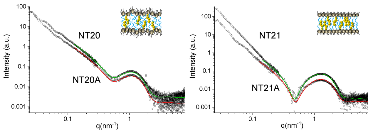
Fig. 1. SAXS spectra of niosomes at 25 °C. Lines represent the fit of the bilayer form factor in the 0.12–8 nm -1 q region for unloaded (green) and ATRA-loaded (red) systems. On the left are reported SAXS spectra for Tween 20 niosomes and on the right are reported the ones for Tween 21 niosomes. (For interpretation of the references to colour in this figure legend, the reader is referred to the web version of this article.)
