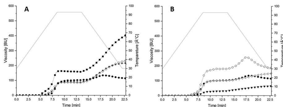
Fig. 2. Visco-amylograph profiles of different flours: —■— corn; —◇— rice; —★— corn-rice-conventional chickpea flour blend (50% w/w corn: rice [3:2] and 50% w/w chickpea flour); —●— conventional chickpea flour; —○— fine chickpea flour; —▼— coarse chickpea flour; —◁— precooked chickpea flour.
