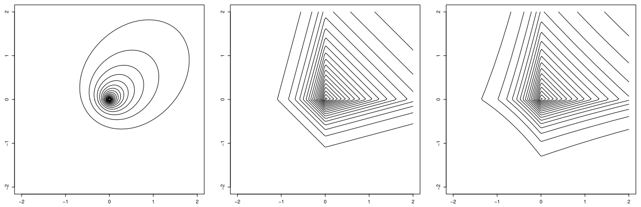
(a) Symmetric, uncorrelated MCAL (b) Symmetric, uncorrelated MSAL (c) Symmetric, uncorrelated MSCAL
