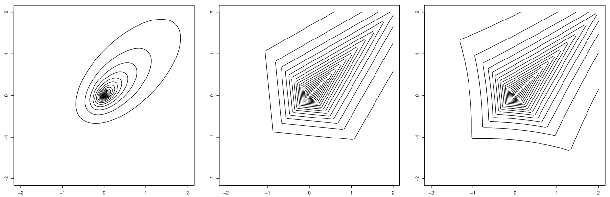
(d) Skewed, uncorrelated MCAL (e) Skewed, uncorrelated MSAL (f) Skewed, uncorrelated MSCAL
