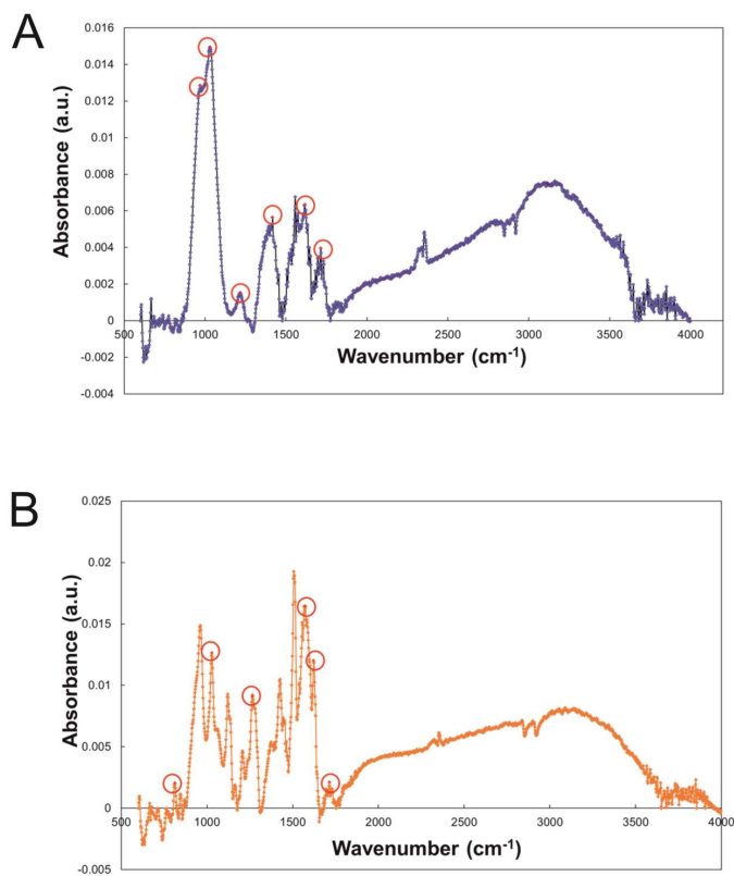
Figure 2. (A) FTIR spectroscopy of GO and (B) GO/CU with characteristic peaks highlighted. The material was directly laid on the ATR crystal, and the spectra were recorded.
