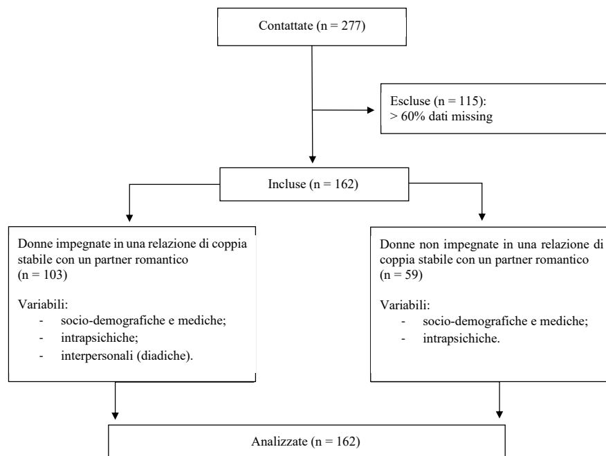
Fig. 2 - Study flowchart
