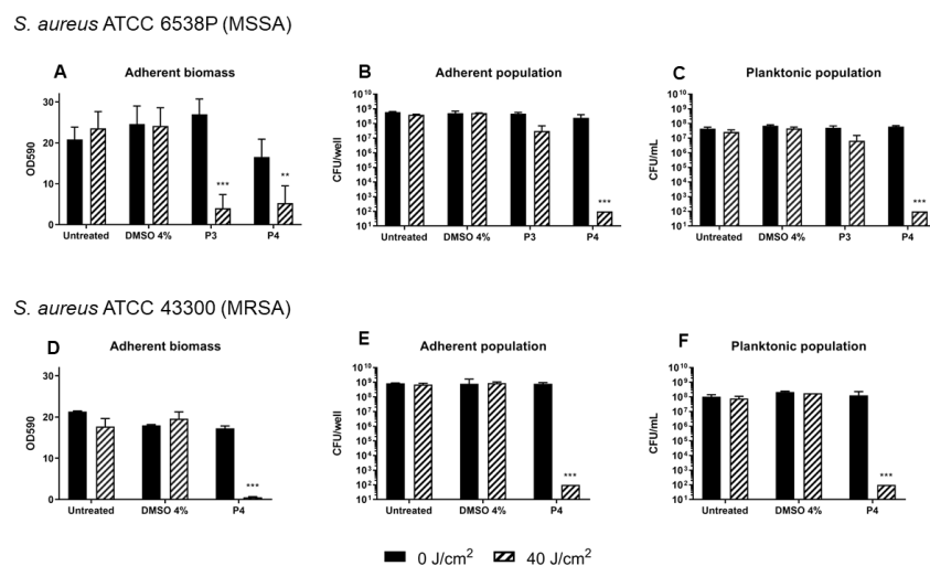
Figure 5. Inhibition of biofilm formation of S. aureus ATCC 6538P (A–C) and ATCC 43300 (D–F) upon photodynamic treatment with diaryl-porphyrin P3 and P4 (20 \mu M). Porphyrins were activated by 410 nm radiation at 40 J/cm 2 . The graphs report values of the optical density at 590 nm (OD 590) after biofilm staining with crystal violet (A,D), values of adherent population density (CFU/well) (B,E), and planktonic population concentration (CFU/mL) (C,F). Dark control samples are represented as black bars and light-treated samples as striped bars. Values represent the mean of at least three independent experiments \pm the standard deviation. Statistical analyses using one-way ANOVA were performed between treated samples and reference untreated control (** p < 0.01 ; *** p < 0.0001 ).
