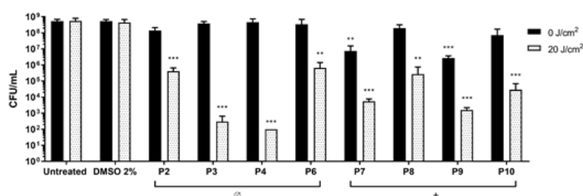
Figure 4. Photodynamic inactivation of S. aureus ATCC 6538P. After 1 h of dark incubation with P2–4, P6, and P7–P10 at 10 µM concentration, cells were irradiated under light at 410 nm at 20 J/cm 2 (grey bars) or kept in the dark (black bars). Values, presented as CFU/mL, are the mean of at least three independent experiments and the bars represent standard deviations. Statistical analyses using one-way ANOVA were performed between treated samples and reference untreated control (** p < 0.01 ; *** p < 0.0001 ).
