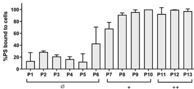
Figure 2. Binding assay of diaryl-porphyrins (P1–P13) to S. aureus ATCC 6538P. Values are presented as a percentage of PS bound to cells upon 1 h of dark incubation. The neutral (Ø), monocationic (+), and dicationic (++) porphyrins were administered at a concentration of 10 \mu M. The experiments were performed in triplicate and standard deviation is reported.
