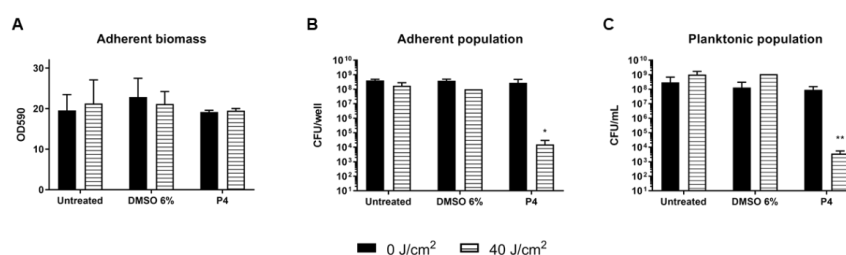
Figure 6. Assay of eradication of S. aureus ATCC 6538P biofilm by porphyrin P4 (30 \mu M) upon irradiation with light at 410 nm (40 J/cm 2 ). Adherent biomass of biofilm upon PDT is represented as OD590 (A) and cell viability is expressed as CFU/well for adherent population (B) and as CFU/mL for planktonic biomass (C). Values represent the mean of at least three independent experiments \pm
