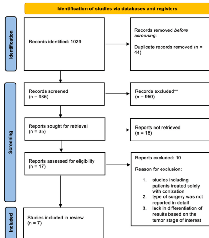
Fig. 1. PRISMA flowchart.
