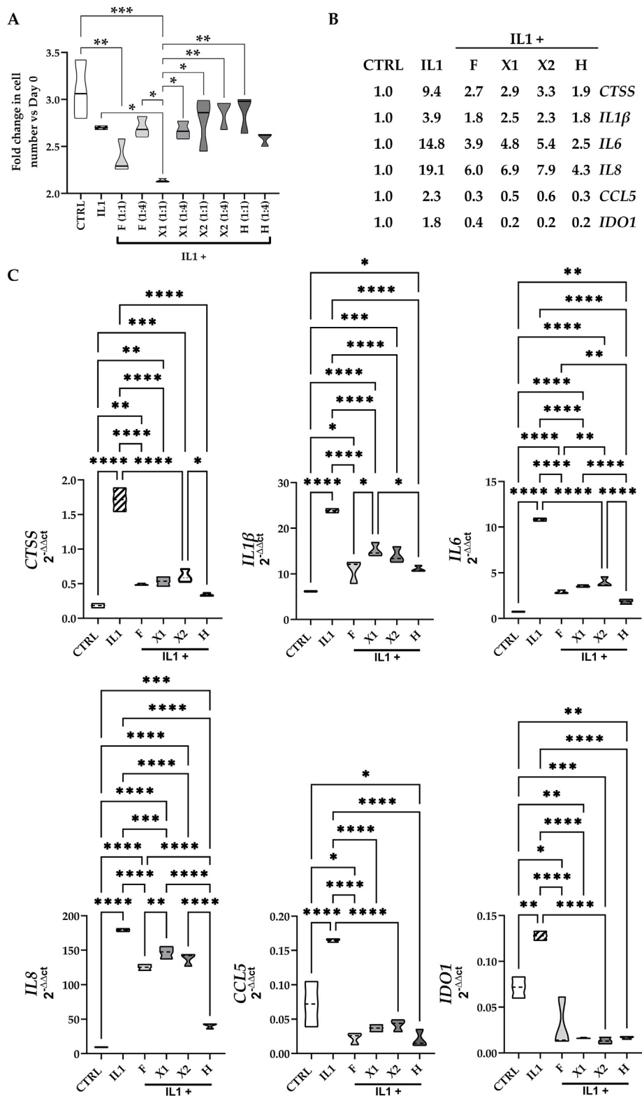
Fig. 5. Effect of secretomes on inflamed chondrocytes. A) Proliferation of chondrocytes exposed to IL1β with or without different dilutions of secretomes. (*p-value \leq 0.05 , ** \leq 0.01 ; N = 3). B) Gene expression modulation (fold change vs CTRL set as 1) for chondrocytes exposed to IL1β without and with secretomes at 1:1 dilution. C) Single gene modulation (*p-value \leq 0.05 , ** \leq 0.01 , *** \leq 0.001 and **** \leq 0.0001 ; N = 3).
