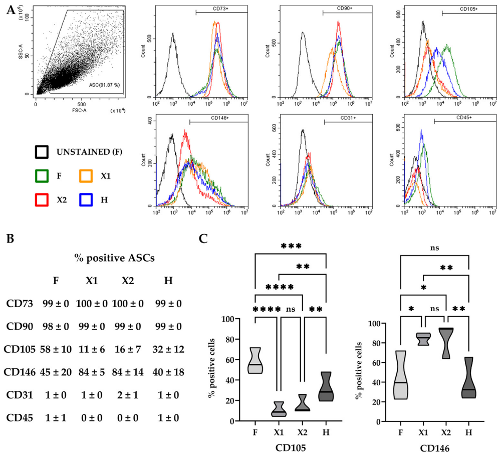
Fig. 1. ASCs immunophenotype. A) Cytograms of markers tested in a representative ASCs cultivated in the four conditions of the study. Unstained sample represents ASCs cultivated in FBS (condition F). B) Percentage of positive ASCs for both MSCs (CD73/90/105/146) and hemato-endothelial (CD31/45) markers (mean ± SD, N = 3 independent experiments). C) Significant differences for CD105 and CD146 between ASCs in the four media. (median (thick line) and 25th and 75th quartiles; *p ≤ 0.05, **p ≤ 0.01, ***p ≤ 0.001, ****p ≤ 0.0001; N ≥ 3 independent experiments).
