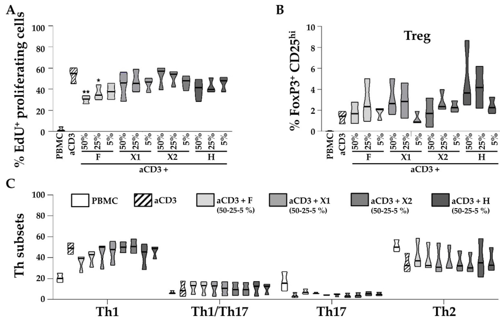
Fig. 6. Immunomodulatory effects of secretomes on PBMC proliferation and T lymphocytes differentiation. A) PBMCs proliferation (*p-value ≤ 0.05, ** ≤ 0.01 vs control (PBMC + anti-CD3), N = 3 independent experiments performed using 3 different PBMC donors and 3 different ASC secretome preparations). B) Treg induction. C) Th subsets differentiation.
