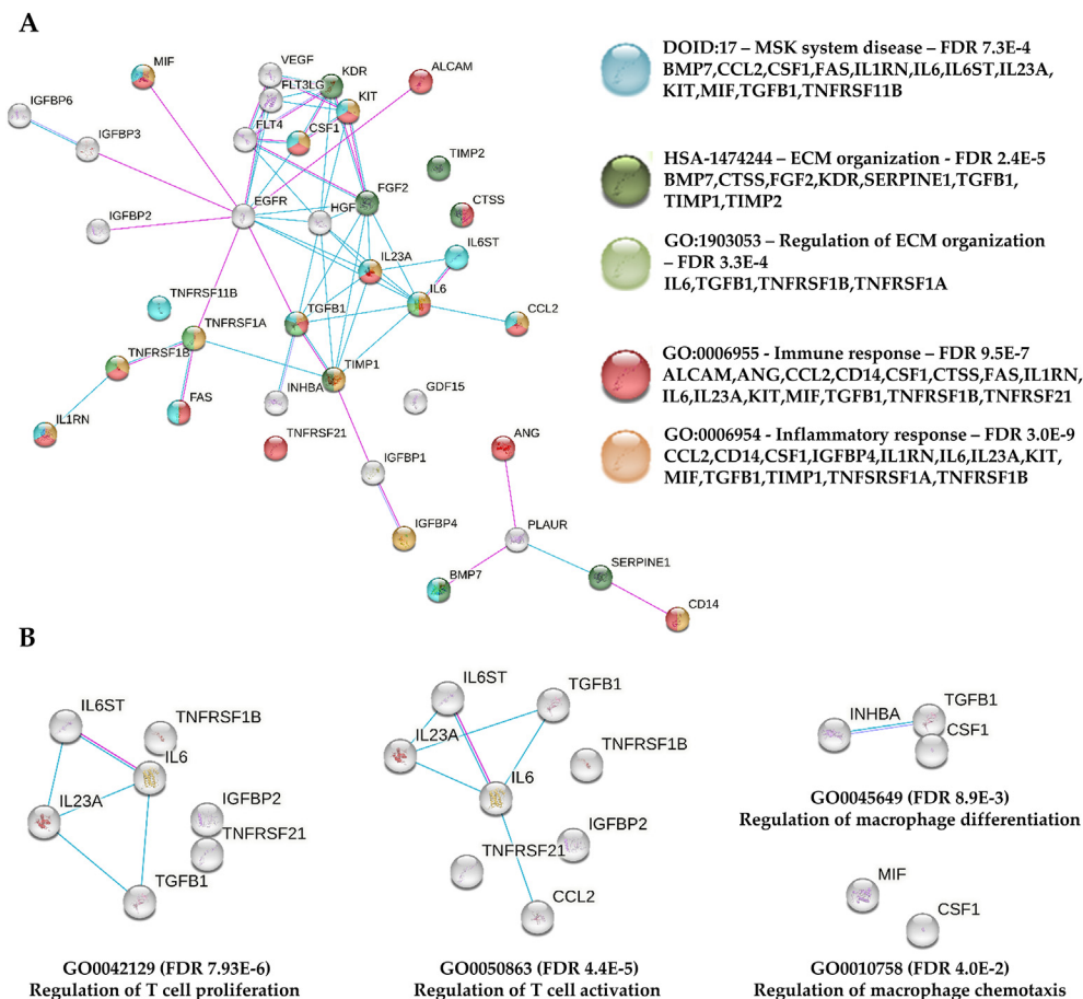
Fig. 2. Functional association network for identified secreted factors. A) Protein–protein interaction levels for 42 proteins shared in ASCs secretome, regardless culture medium, mined using STRING. Blue connections = proteins with known interactions based on curated databases; violet connections = proteins with experimentally determined interactions. Colourless nodes = proteins not related to the terms: MSK system disease, ECM organization, regulation of ECM organization, immune or inflammatory response. False discovery rate (FDR) for each term is also shown. Empty nodes = proteins of unknown 3D structure; filled nodes = known or predicted 3D structure. B) Protein–protein interaction networks for proteins belonging to regulation of T cell proliferation, activation and of macrophage differentiation, chemotaxis.
