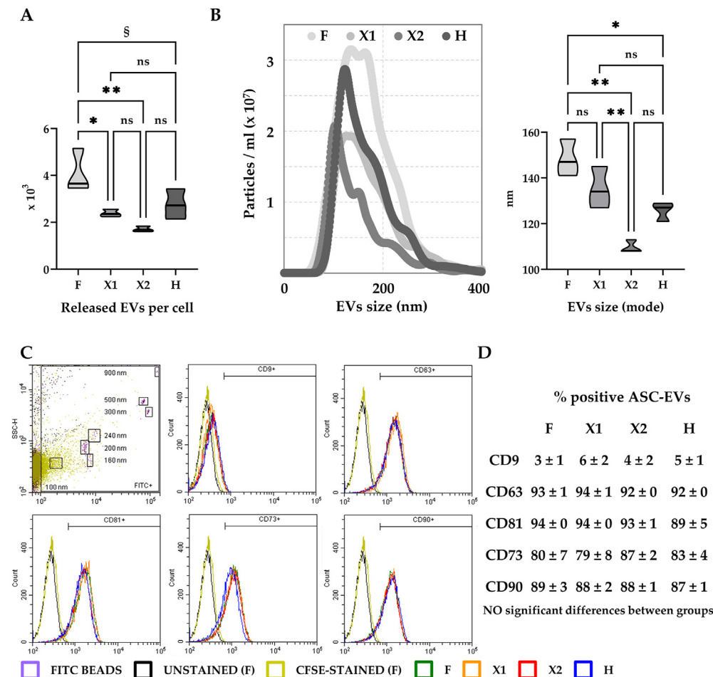
Fig. 3. ASC-EVs characterization. A) EVs released per cell calculated from NTA data. (median (thick line) and 25th and 75th quartiles, ^{\S}p \leq 0.10 , ^*p \leq 0.05 , ^{**}p \leq 0.01 ; N \geq 3 independent experiments). B) EVs size analysis between conditions using NTA (each curve was obtained merging the data from three independent ASC lines). Mode size results are displayed as violin plots showing median (thick line) and 25th and 75th quartiles ^*p \leq 0.05 , ^{**}p \leq 0.01 ; N \geq 3 independent experiments). C) Representative cytograms of EVs (CD9/63/81) and MSCs (CD73/90) markers tested in a representative ASC-EVs and superimposed in the dot plot with FITC-positive calibration beads of predetermined size (100, 160, 200, 240, 300, 500 and 900 nm) to confirm reliability of particle detection in the nanometric range. Unstained and CFSE stained samples represents only EVs from ASCs cultivated in FBS (condition F). D) Percentage of positive EVs for each marker (mean \pm SD, N = 3 independent experiments).
