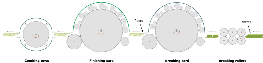
Fig. 4. Schematic representation of the extraction stage by carding route (from right to left).
