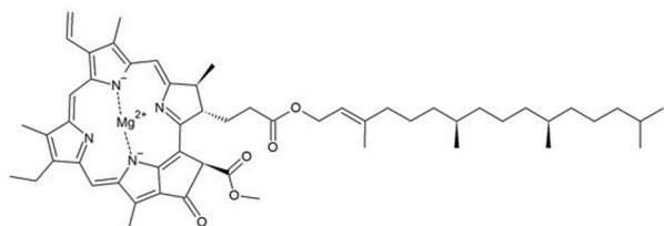
Bacteriochlorophyll a
