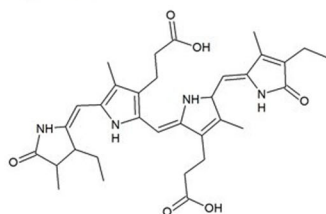
Phycocyanobilin
