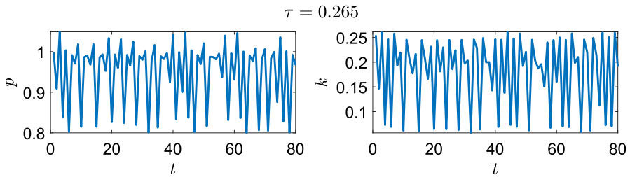
Fig. 3 Time series obtained for \theta = 1.5 and \gamma = 2 , showing chaotic endogenous oscillations. (Color figure online)
