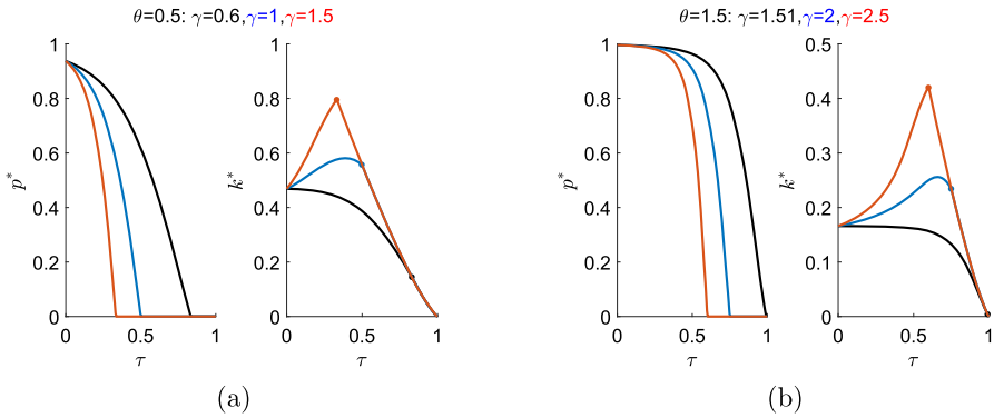
Fig. 2 Comparative statics of p^* and k^* with \beta < 1 for small (panel a) and large (panel b) values of \theta . Related to Corollary 1, black, blue and red colors are respectively used for scenario (i), (ii) and (iii). The small circles in each graph of k^* represent points at which \tau = \theta/\gamma . (Color figure online)
