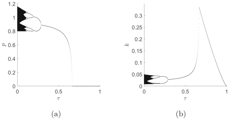
Fig. 8 Bifurcation diagrams for variable p (left column) and k (right column)
