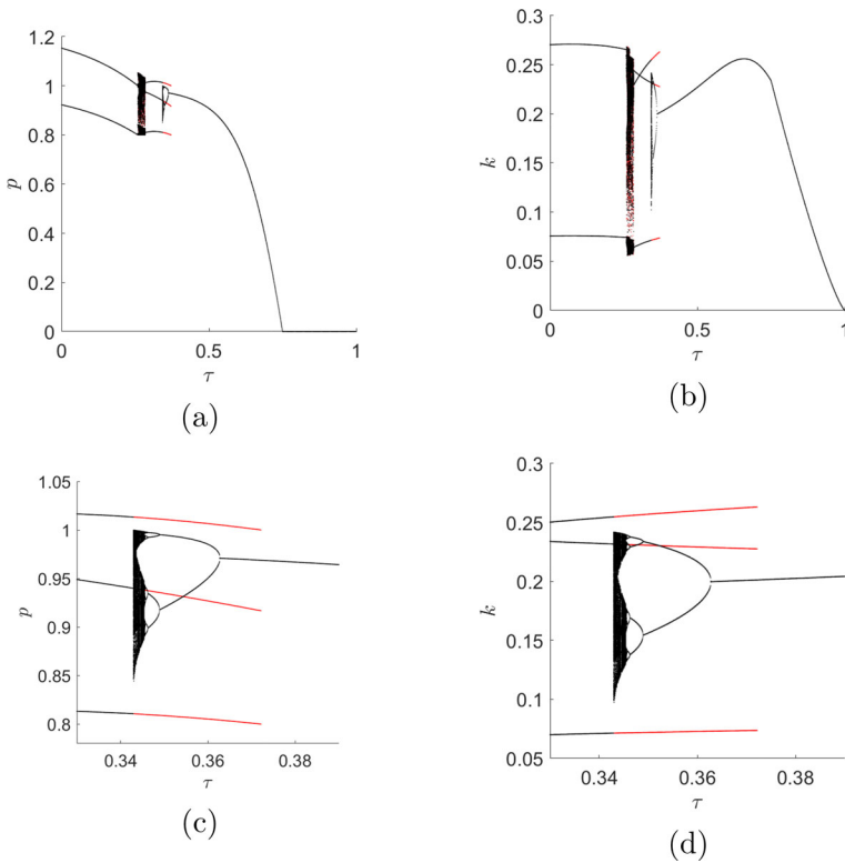
Fig. 4 Bifurcation diagrams for variable p (left column) and k (right column). Different initial data are considered, showing the coexistence of distinct attractors (red and black bifurcation diagrams). In the top row \tau ranges over the entire interval [0, 1) , whereas in the bottom row we report a blow up on the interval (0.33, 0.39) . (Color figure online)
