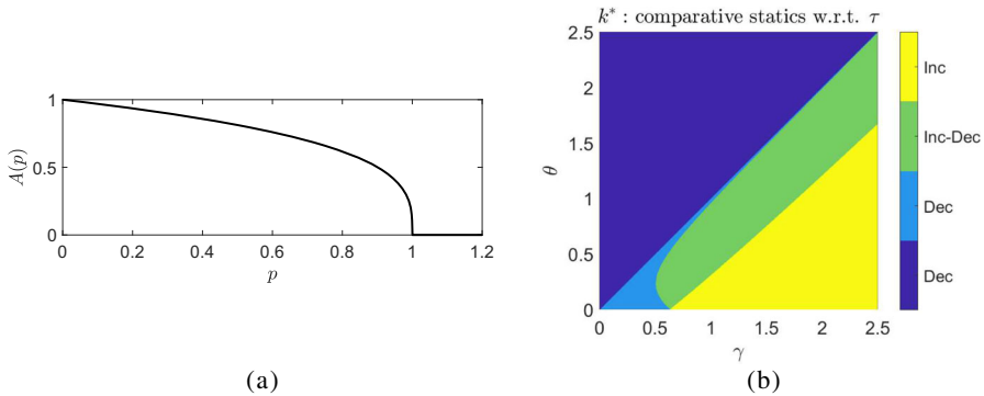
Fig. 1 a Graph of function (12) for \beta < 1 . b Regions of the parameter space (\gamma, \theta) in which we have different monotonicity behaviors of k^* as \tau increases. Light blue, green and yellow colors respectively represent scenarios (i),(ii) and (iii) of Corollary 1, while dark blue region corresponds to \gamma \leq \theta . (Color figure online)
