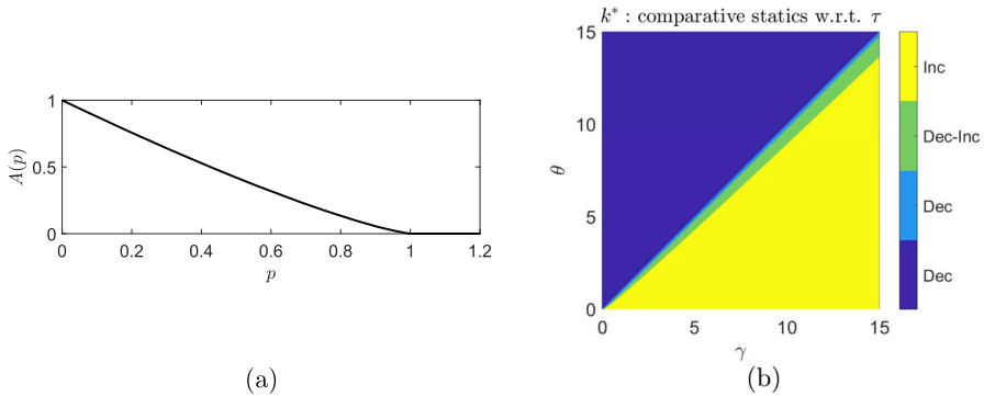
Fig. 6 a Graph of function (12) for \beta > 1 . b Regions of the parameter space (\gamma, \theta) in which we have different monotonicity behaviors of k^* as \tau increases. Light blue, green and yellow colors respectively represent scenarios (i),(ii) and (iii) of Corollary 3, while dark blue region corresponds to \gamma \leq \theta . (Color figure online)
