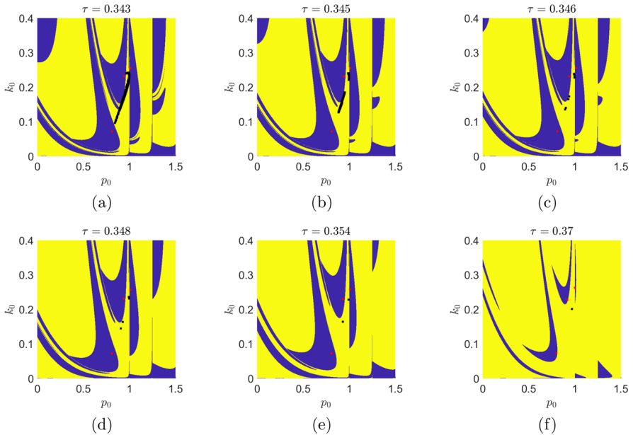
Fig. 5 Basins of attraction related to the attractors shown in the bifurcation diagrams of Fig. 4, for different values of \tau . The blue region is the basin of the period-3 cycle (depicted in red), while the yellow region is related to the black attractor. (Color figure online)
