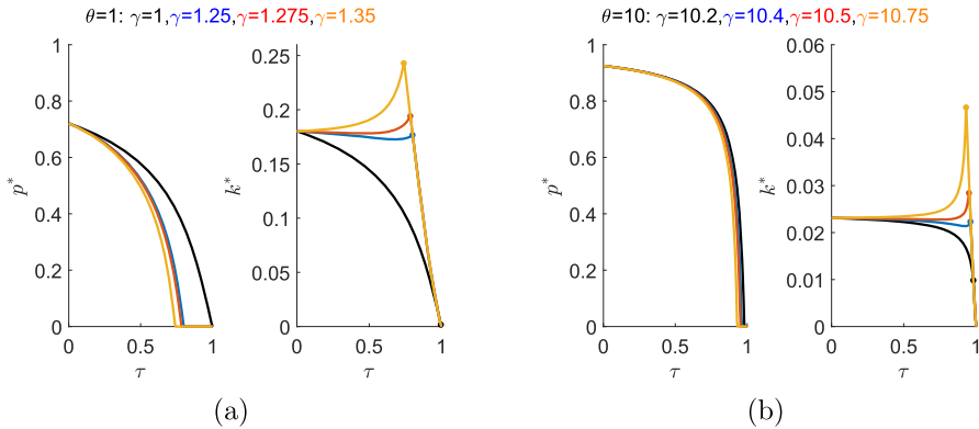
Fig. 7 Comparative statics of p^* and k^* with \beta > 1 for small (panel a) and large (panel b) values of \theta . Related to Corollary 3, black and yellow colors are respectively used for scenario (i) and (iii), while blue and red colors are used for two different situations related to scenario (ii). The small circles in each graph of k^* represent points at which \tau = \theta/\gamma . (Color figure online)
