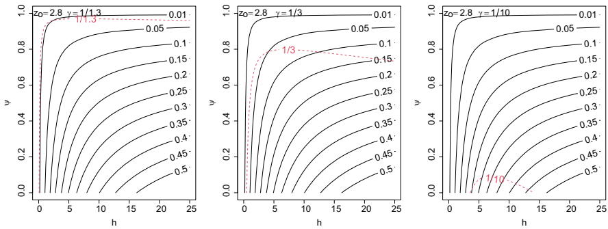
Fig. 1 \alpha -contours of p -values for prior-data conflict (solid black line). Contour for BF_{0:SM}(\hat{\theta}_o; \psi, h) = \gamma (dashed red line), for z_o = 2.8 and three selected values of \gamma . The intersection between the p -value at level \alpha and the BF_{0:SM} at level \gamma yields the pair of solutions (\psi_{\gamma,\alpha}, h_{\gamma,\alpha}) (color figure online)
